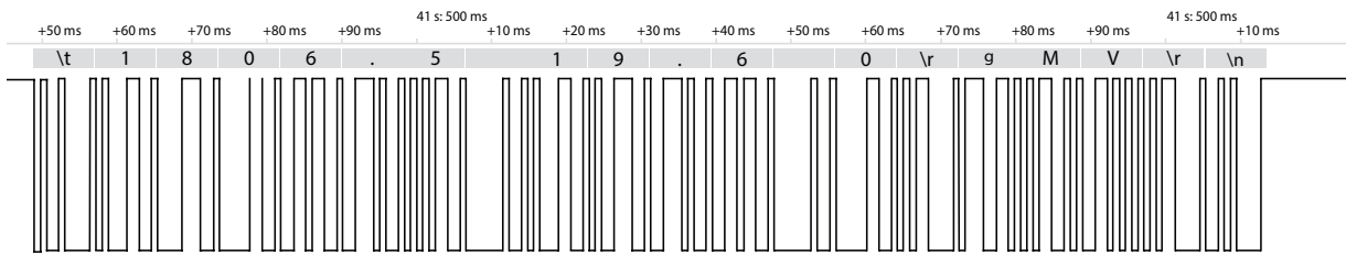
Figure 7 Example DDI Serial transmission
